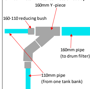
Tank bank return water connection outlay
