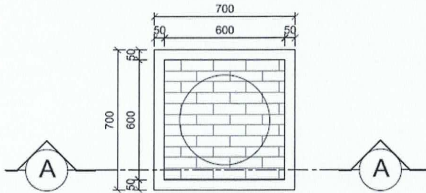
PLAN SCALE 1:20
