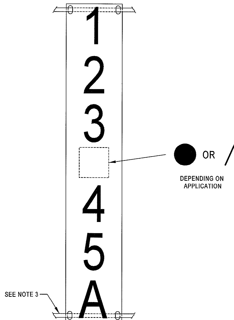
NUMBER PLATE WITH UNIQUE NUMBER AND 'BAND-IT' STRAPS
