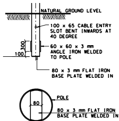
BASE PLATE DETAIL
