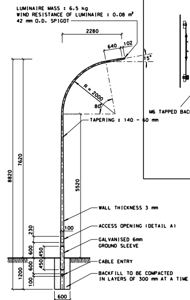
STANDARD POLE FOR 125W MV AND 70W HPS LUMINAIRES
