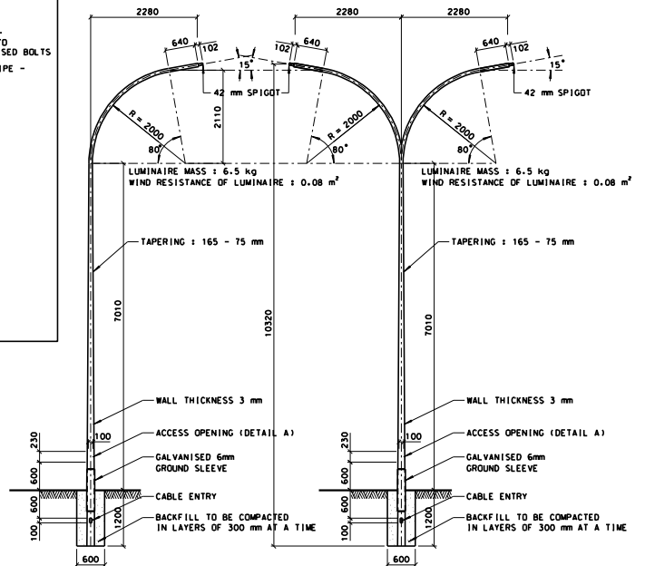
STANDARD POLE FOR 400W MV AND 250W HPS LUMINAIRES
