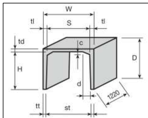
Reinforced Concrete Rectangular Portals
