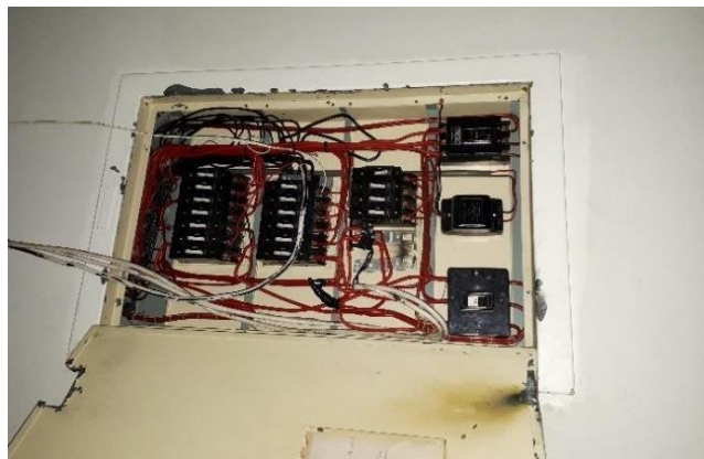
Photo 4: Informal electrical connections
