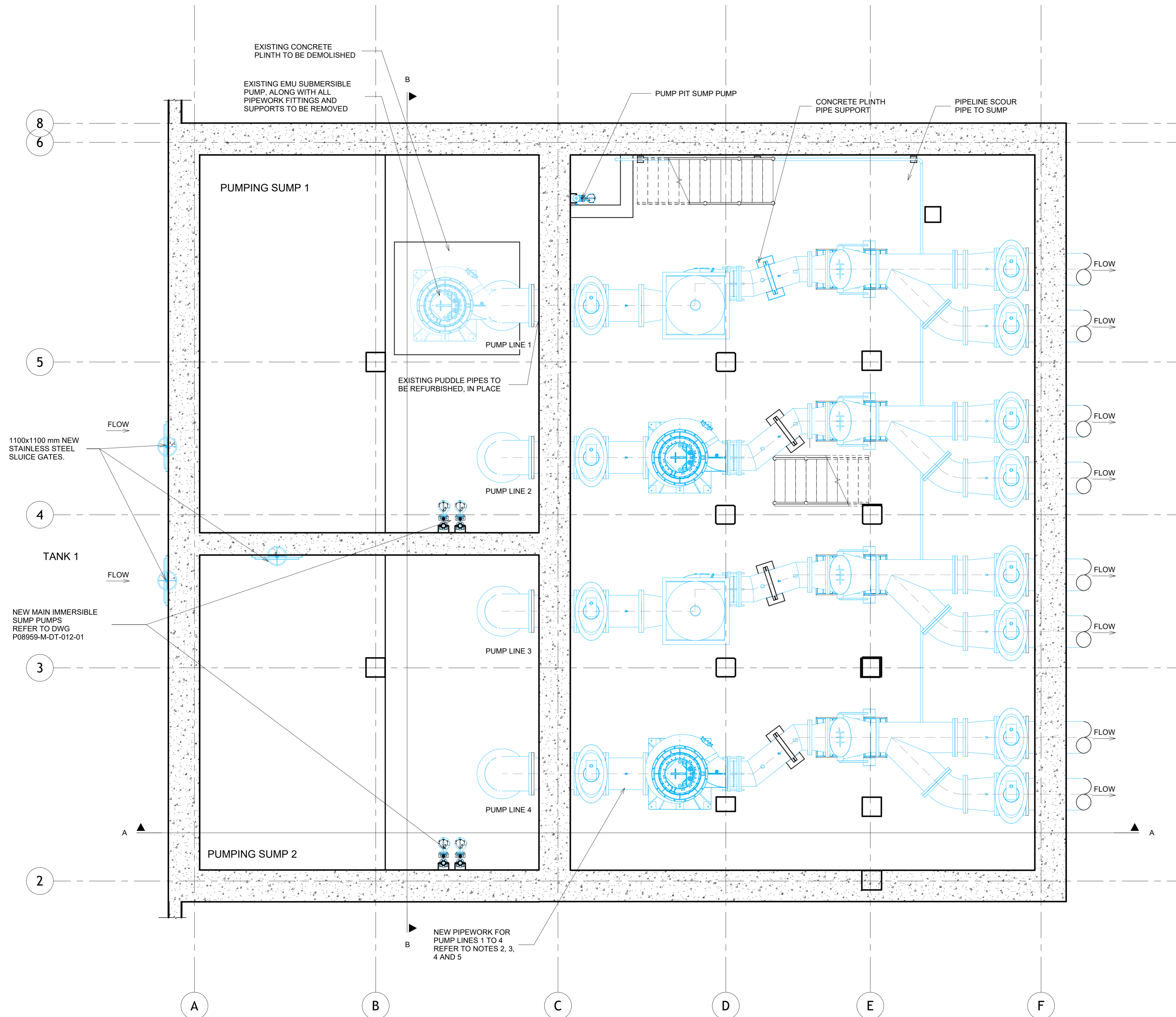
PLAN VIEW 1 : 50
