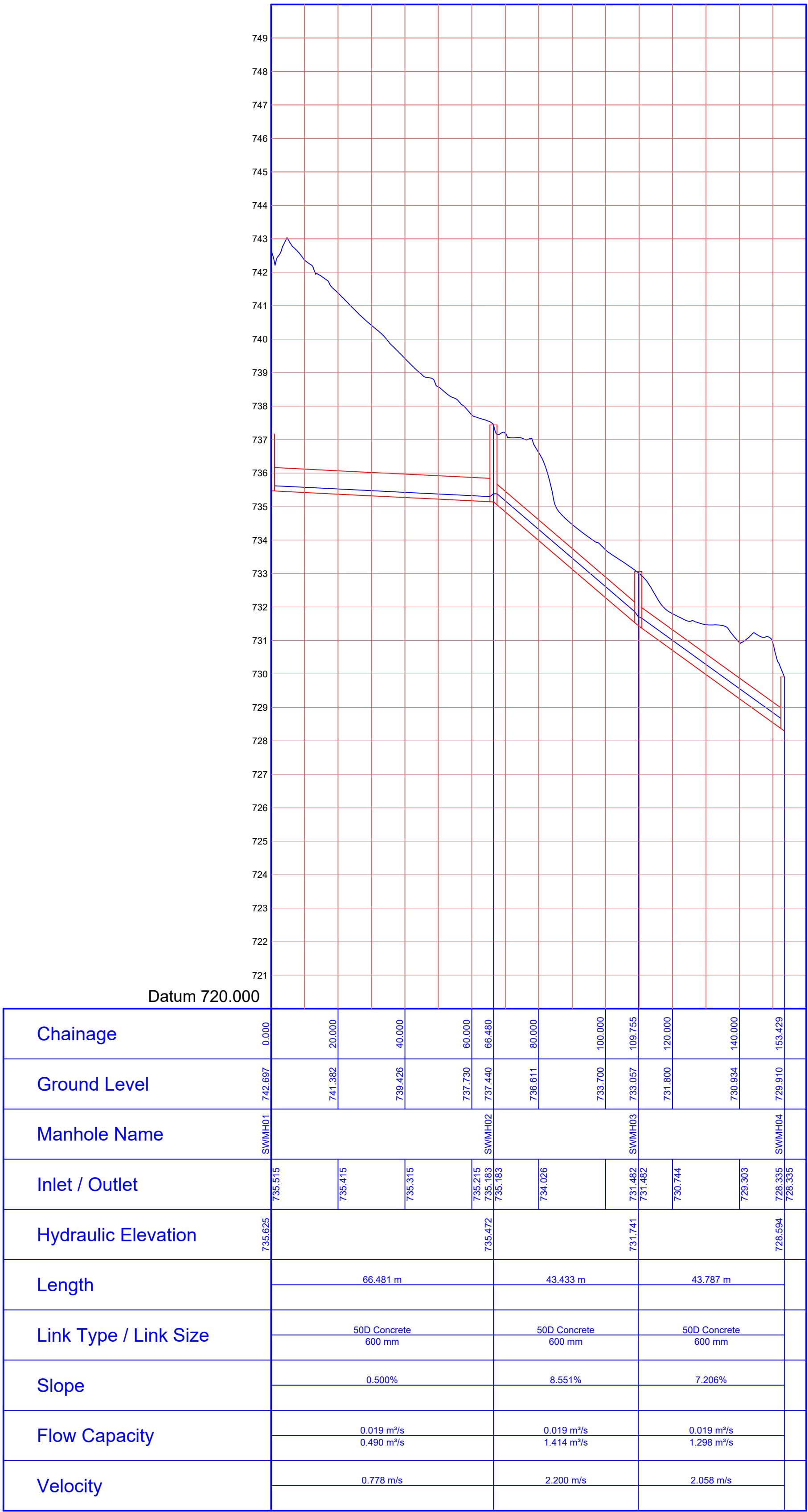
Manhole SWMH01 to SWMH04
