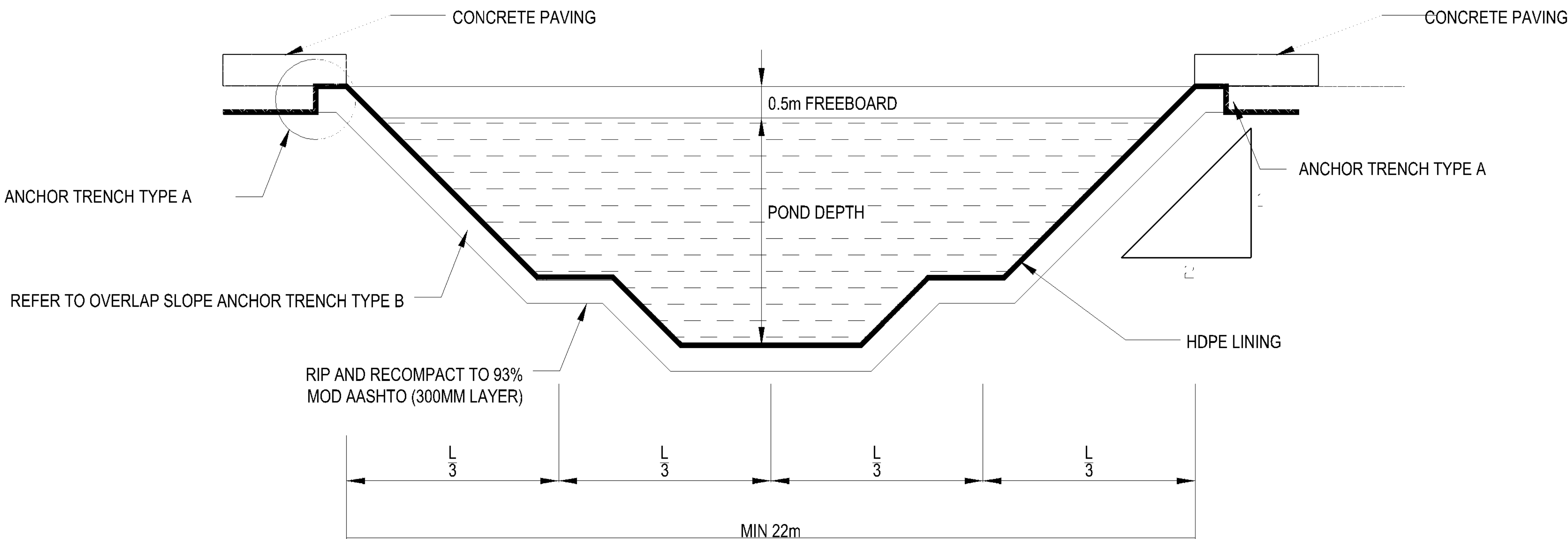
CROSS-SECTION THROUGH A NEW POND SECTION A-A
