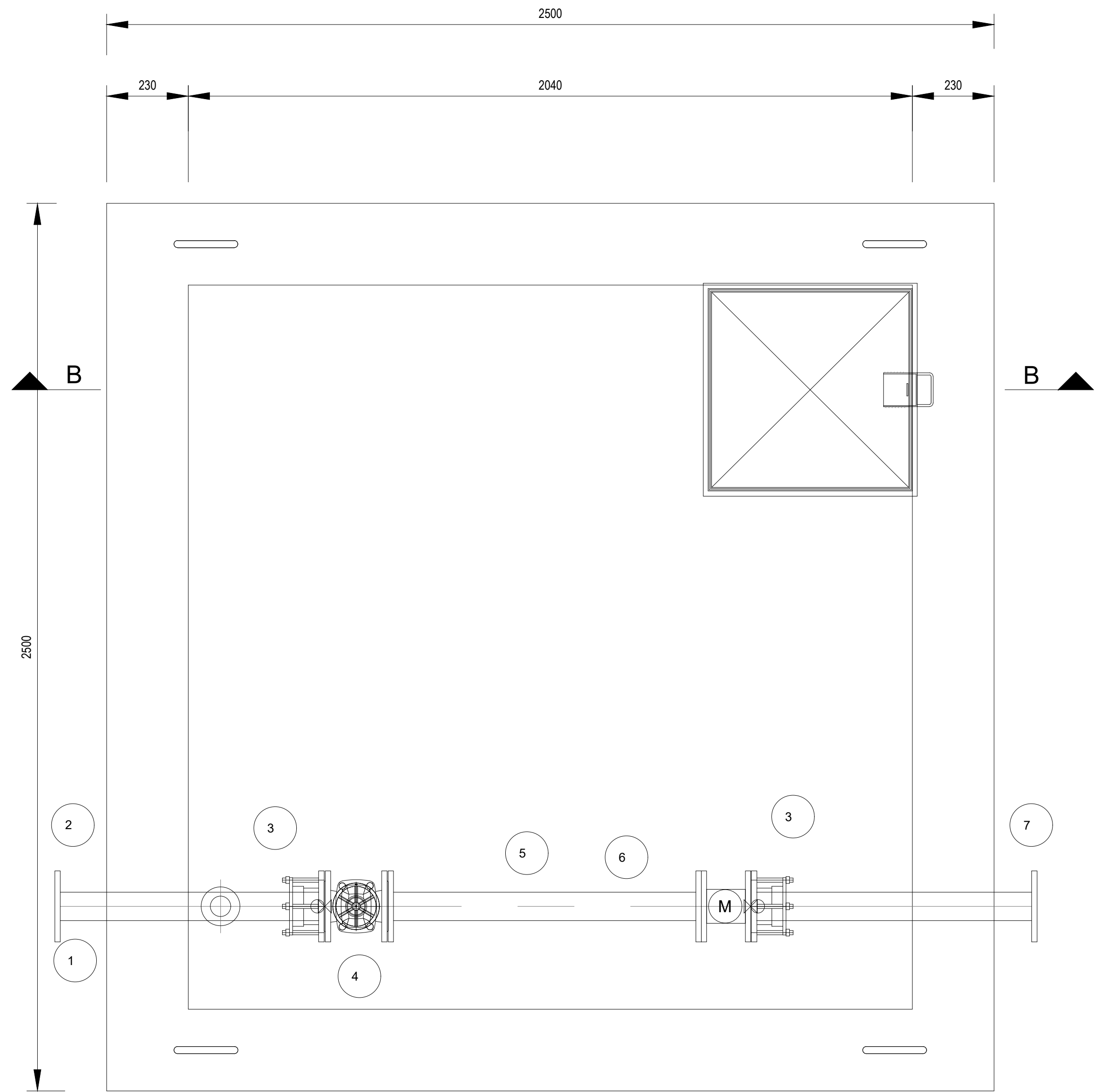
PLAN
