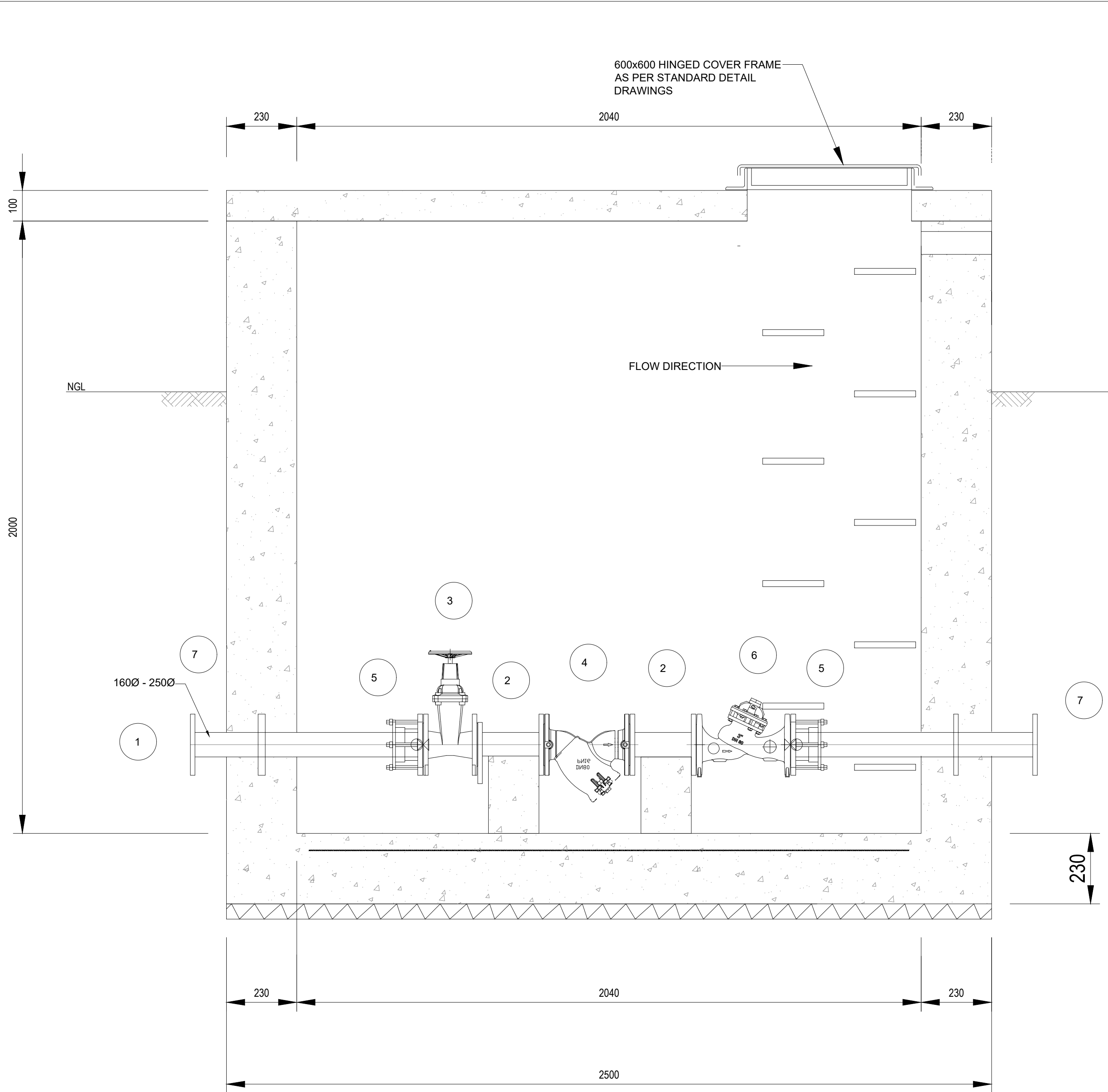
SECTION B-B INLET CHAMBER[DN160mm - 250mm] SCALE 1 : 10
