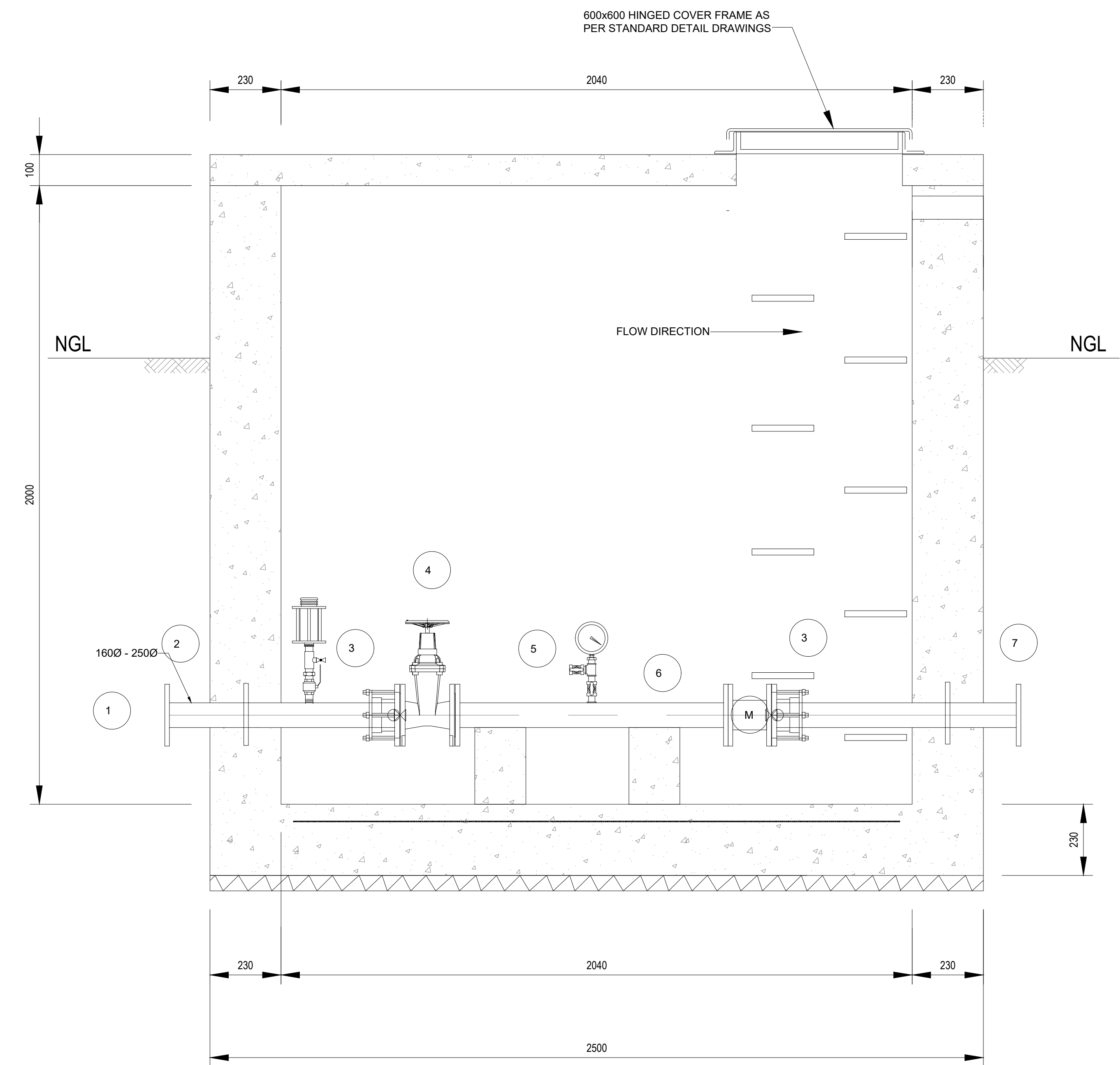
SECTION B-B OUTLET CHAMBER[DN160mm - 250mm]
