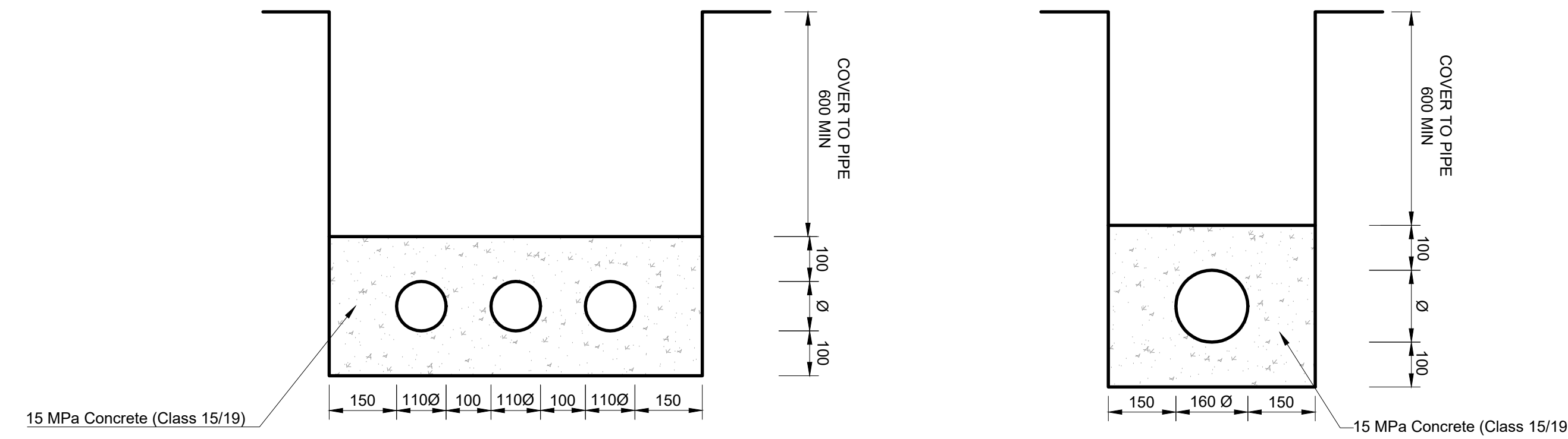
SLEEVE DUCTS CONCRETE ENCASEMENT DETAILS SCALE - NTS
