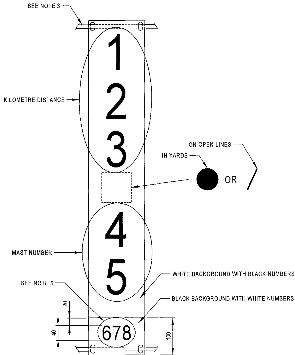
NUMBER PLATE WITH UNIQUE NUMBER (TO BE ATTACHED WITH 'BAND-IT' STRAPS)
